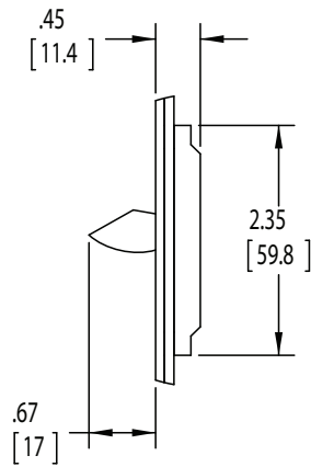
Tongue Detail
