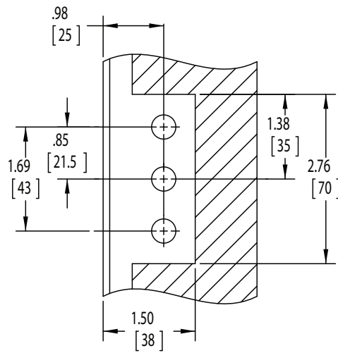
Mortise Prep
